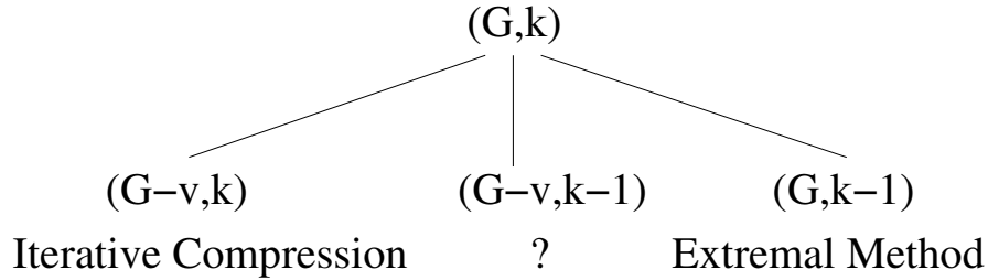
Figure 10: Three ways, of which only two correspond to known techniques, to design an FPT algorithm by induction.
