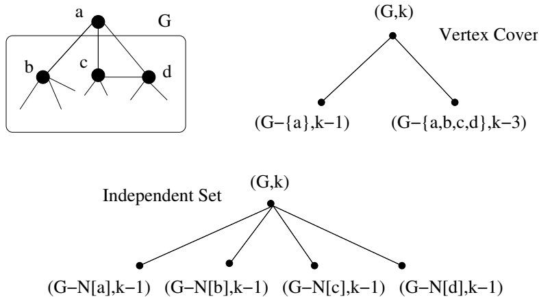
Figure 3: Illustrating Observations 2 and 3. A graph G with vertex a having 3 neighbors, and two levels of the bounded search trees for k -Independent Set in Planar Graphs and for k -Vertex Cover. Any maximal independent set will contain either vertex a or at least one of its neighbors, while any vertex cover will contain either vertex a or all 3 neighbors.
