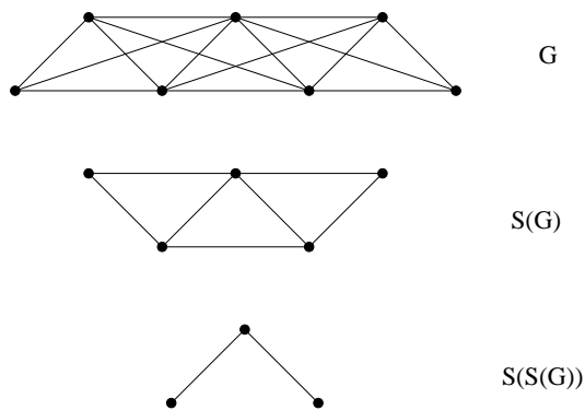
Figure 1: The 3-ray on 7 vertices (a graph in C_{2,2} ), its separator graph the 2-ray on 5 vertices (a graph in C_{2,1} ), and its separator graph the 1-ray on 3 vertices (a graph in C_{2,0} ).
