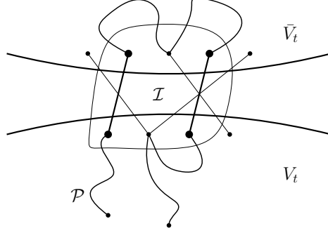
Figure 1: The intersection of an induced path \mathcal{P} with G[V_t \cup \text{bd}(\bar{V}_t)] , which is an induced disjoint union of paths \mathcal{I} . The subgraph S to be used as an index for the corresponding table entry consists of the boldface vertices and edges in \mathcal{I} .
