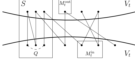
Figure 2: A crossing graph G_{t, \bar{t}} and the structures associated with the table indices of the algorithm for LONGEST INDUCED PATH. Note that by (iv) and (i) it follows that if the table entry corresponding to the above structures is 1, then j = 0 : Since both degree one endpoints in S[V_t] are paired, this means that the corresponding set of induced paths \mathcal{I} has zero degree one endpoints in G[V_t] .
