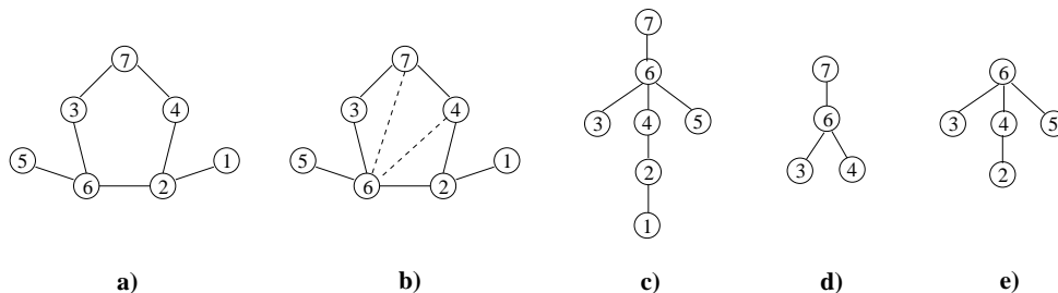
Figure 1: A graph G with a given order \alpha is shown in a), and b) shows G_\alpha^+ . The corresponding elimination tree ET and the pruned subtrees ET_p[7] and ET_p[6] are given in c), d), and e), respectively.
