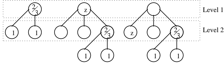
Figure 5: Illegal colorings by Claim 3 if z \in \{4, 5, 6\} .
