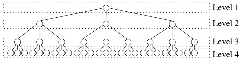
Figure 4: An example of T_4^- .
