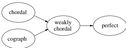
Fig. 1. The inclusion relationship between the graph classes mentioned in this paper. The \rightarrow represents the \subset relation between the classes.
