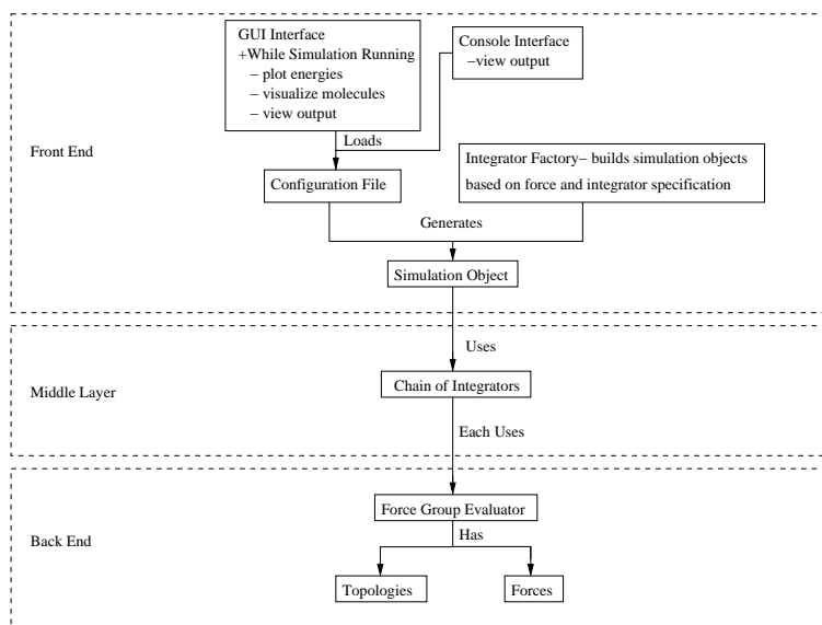
Fig. 2. Snapshot of the flow of execution in a typical MD simulation using PROTOMOL
