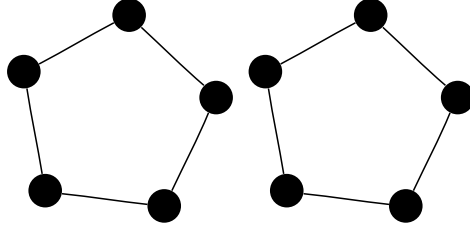
Fig. 3: The “Double 5-Cycle” Graph
