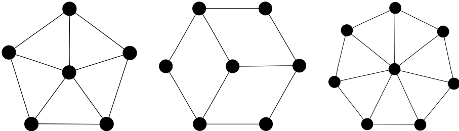
Fig. 4: Circle Graph Obstructions
