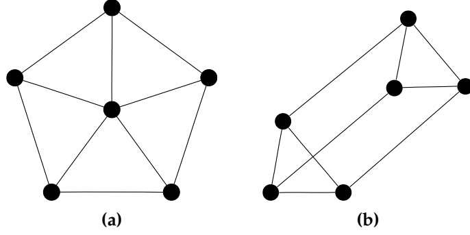
Fig. 1: Two Graph Representations of the Hexacode
