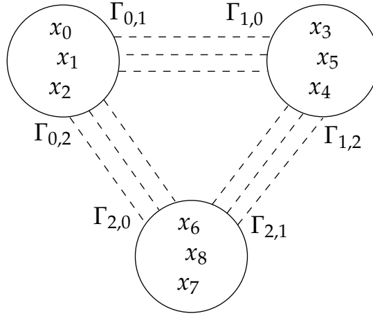
Fig. 6: Example of Construction with Low PAR_{IHN}
