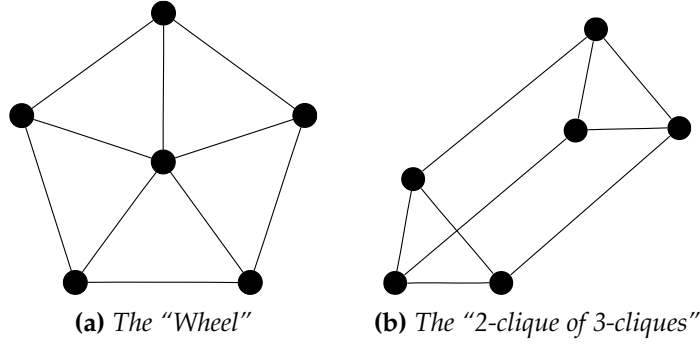
Fig. 1: The LC Orbit of the [[6,0,4]] Hexacode
