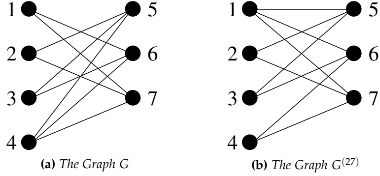
Fig. 3: Two Graph Representations of the [7,4,3] Hamming Code
