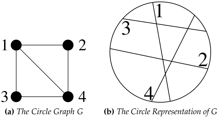
Fig. 3: Example of a Circle Graph
