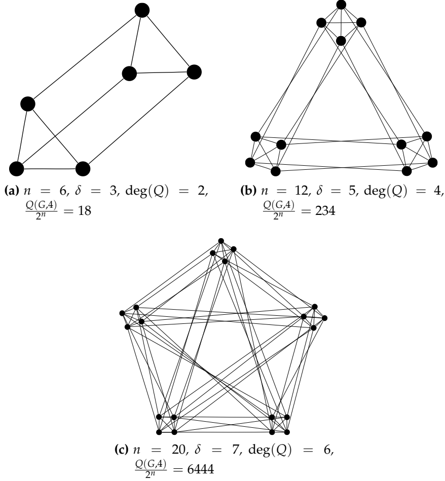
Fig. 7: Examples of Nested Clique Graphs
