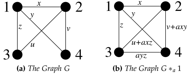
Fig. 3: Example of Generalized Local Complementation
