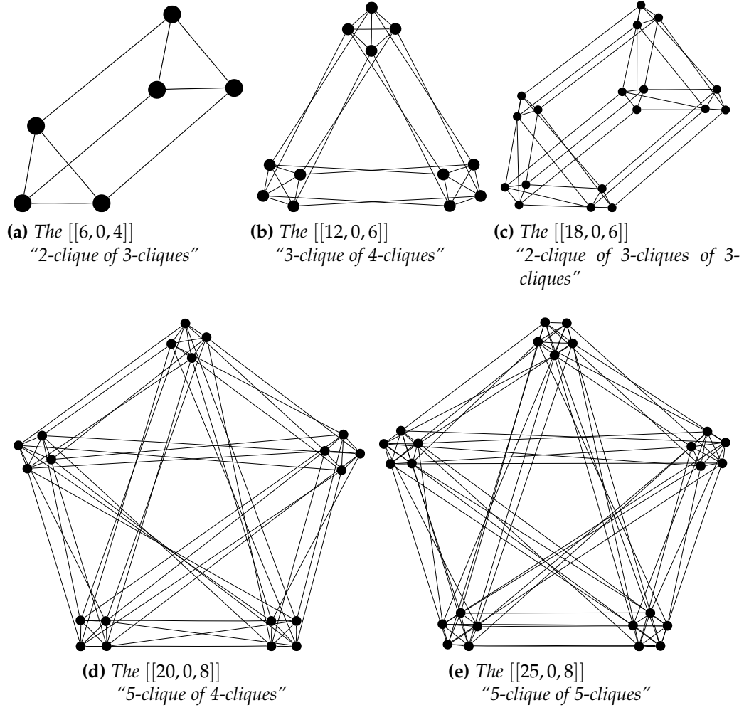
Fig. 2: "Nested Clique" Graphs
