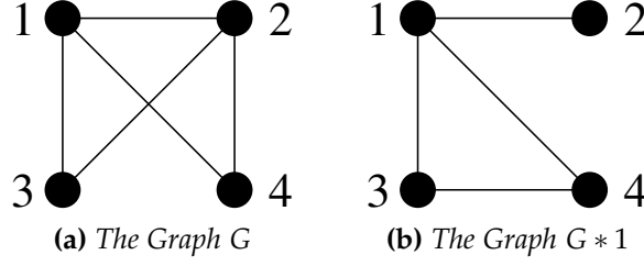
Fig. 2: Example of Local Complementation
