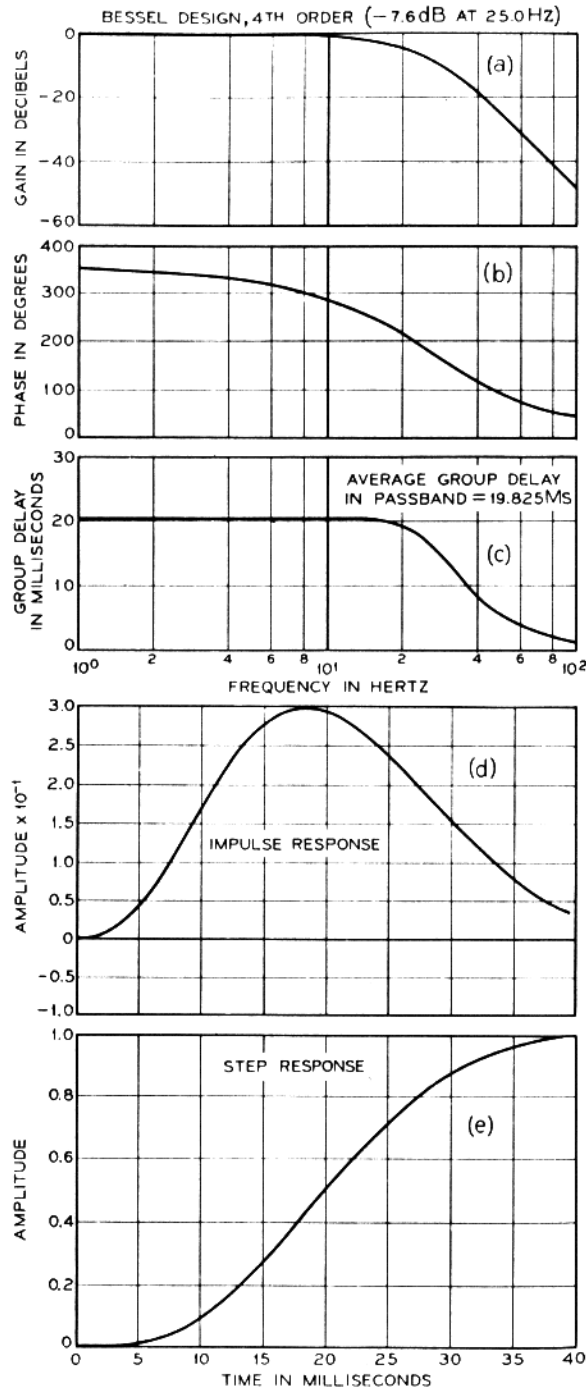
Fig. 5 — Fourth-order Bessel low-pass filter used to smooth the |F_n| and \dot{\phi}_n signals.
