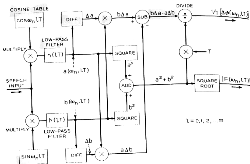
Fig. 3 — Programmed operations for extracting |F(\omega_n, l)| and \phi(\omega_n, l) .
