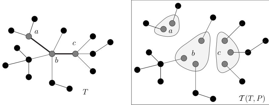
Fig. 1. An example of the definition of the graph collection \mathcal{T}(T, P) for some tree T and some path P = (a, b, c) in it.
