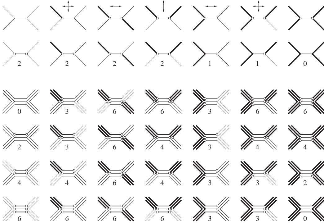
Fig. 7. There are 16 possible ways shadow edges can be distributed around an edge e with both endpoints of degree 3. We present 7 representative configurations (the rest come up as symmetric ones – arrows depict the symmetries) and the way the sub-ordering e^1, e, e^2 is contributing to the linear-width of L^* . Notice that, in each case, the contribution of the endpoints of e^1, e, e^2 in L^* is never more than 3 times the contribution of the endpoints of e in L .
