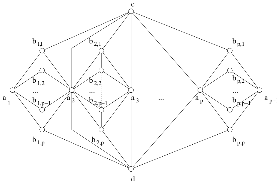
Figure 2: Planar graphs with many large potential maximal cliques
