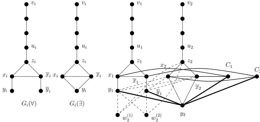
Figure 1: Graphs G_i(\forall) , G_i(\exists) and G for \phi = \forall x_1 \exists x_2 (x_1 \vee \bar{x}_2) \wedge (\bar{x}_1 \vee x_2) , f = 3 . The edges shown by dashed lines are used to force the players to move in a special way.
