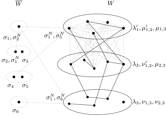
Figure 4. An illustration; graph G_2 of maximum degree 3 constructed for H (the dotted edges) from Figure 3, and the resulting labelling of V(G_2) = W \cup \overline{W} , as in the proof of Theorem 3.7.
