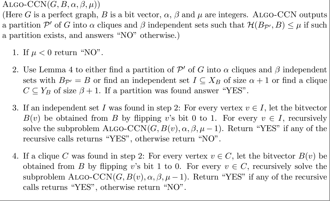
Figure 1: Description of Algorithm ALGO-CCN
