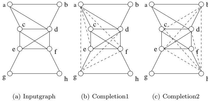
Figure 3: Given the input graph G = (V, E) , we can find at least two different maximum independent sets: M_1 = \{b, c, h\} and M_2 = \{a, f, g\} . In fig. 3(b) we make V \setminus M_1 in a clique adding 5 edges; In fig. 3(c) we make V \setminus M_2 in a clique adding 6 edges. This means that even taking a maximum independent set, we cannot be sure to get a minimum completion.
