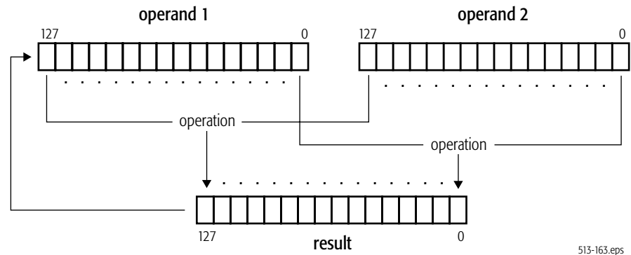
Figure 4-25. Arithmetic Operation on Vectors of Bytes
