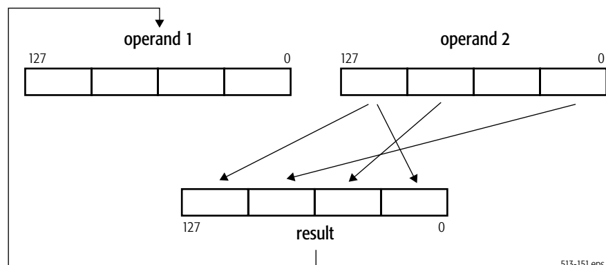
Figure 4-5. Shuffle Operation
