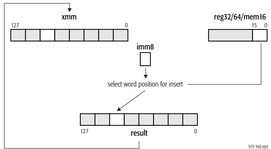
Figure 4-22. PINSRW Operation
