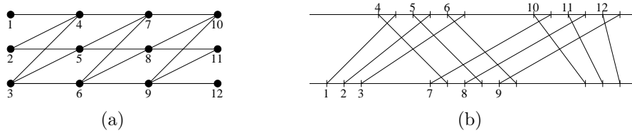
Figure 4: (4 \times 3) Hsu-stable chain (a) and its permutation representation (b).
