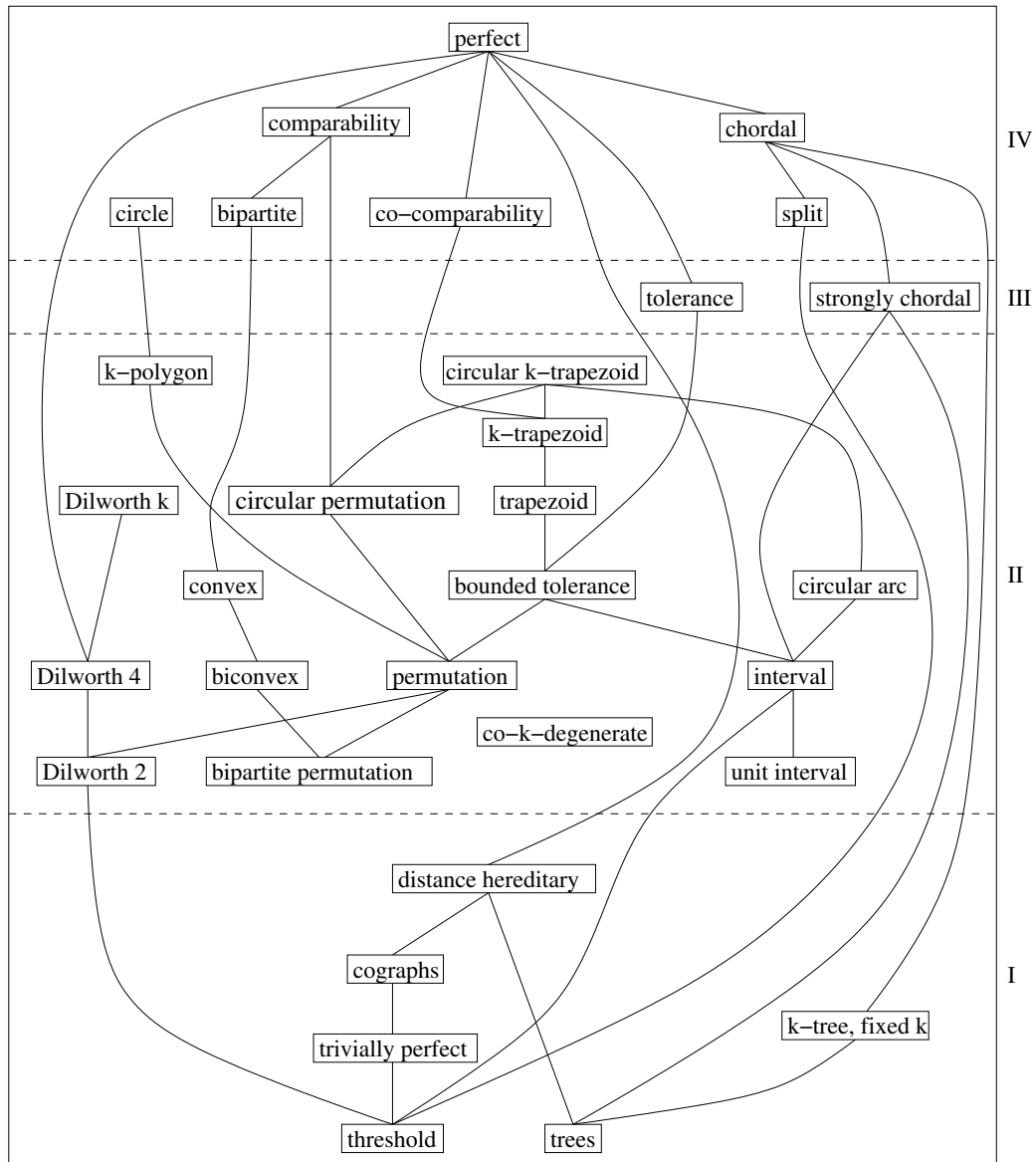
Figure 4.5: Inclusion diagram of some well-known graph classes.
