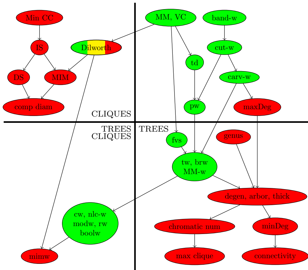
Figure 5.2: The parameterized complexity of \text{MSOL}_1 problems. Red means there exists an \text{MSOL}_1 problem which is para-NP-hard and green means all \text{MSOL}_1 problems are FPT. The complexity parameterized by Dilworth number is open.
