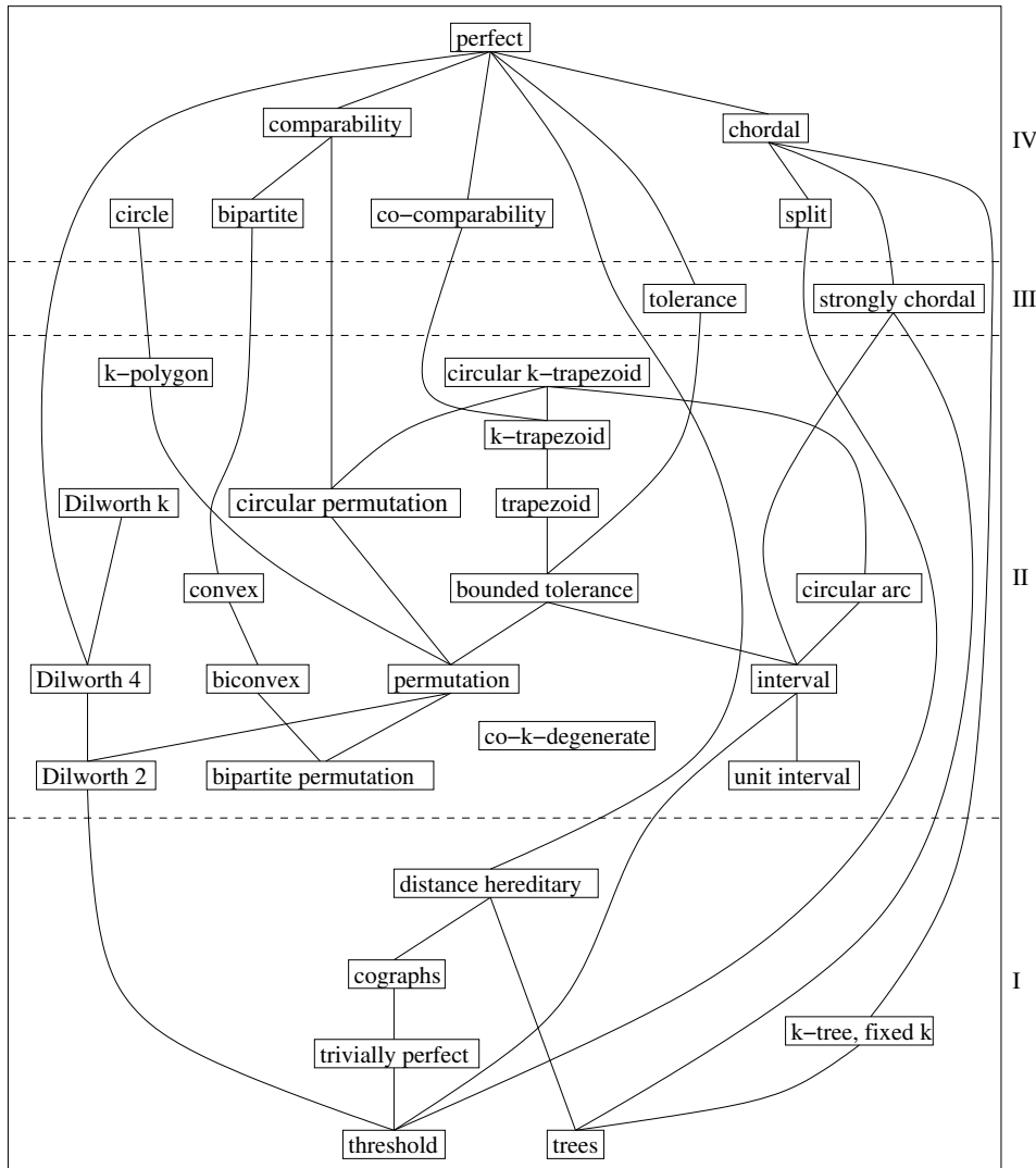
Figure 1: Inclusion diagram of some well-known graph classes.
