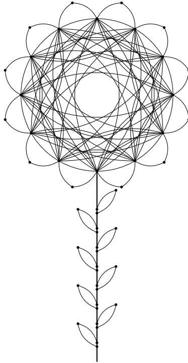
Figure 1: The Sunflower graph
