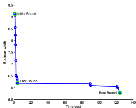
Figure 2: Improvement of boolean-width upper bound as the local search progresses over time, for the graph eil51.tsp ( V=51, E=140 )
