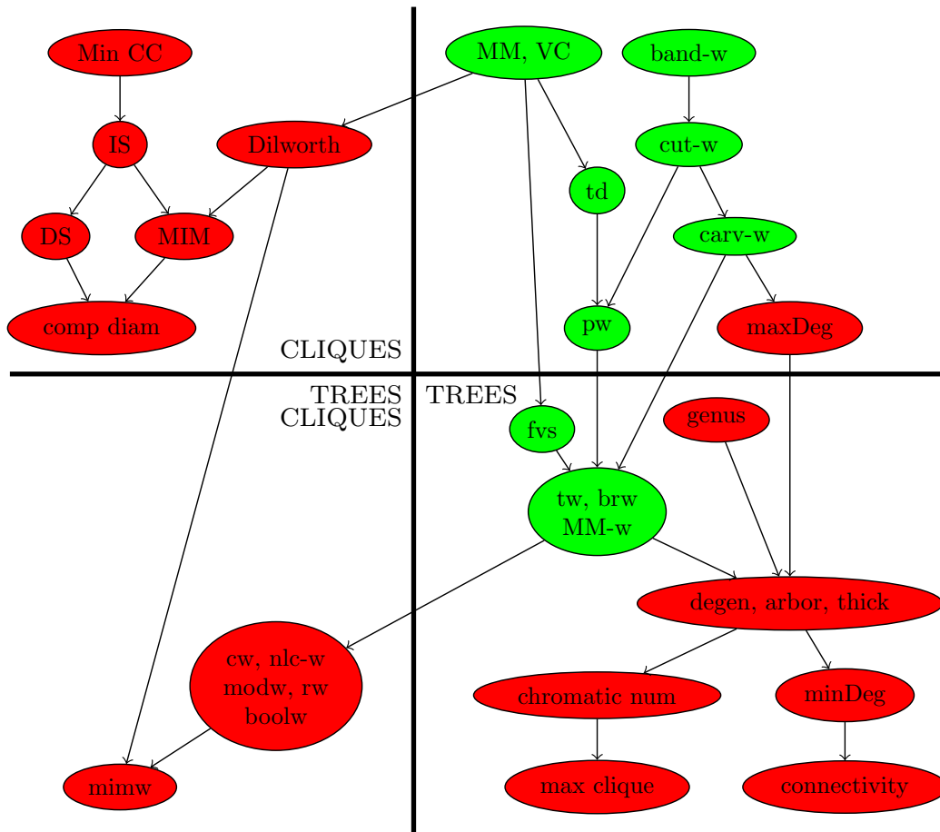
Figure 5.1: The parameterized complexity of MSOL_2 problems. Red means there exists an MSOL_2 problem which is para-NP-hard and green means all MSOL_2 problems are FPT.
