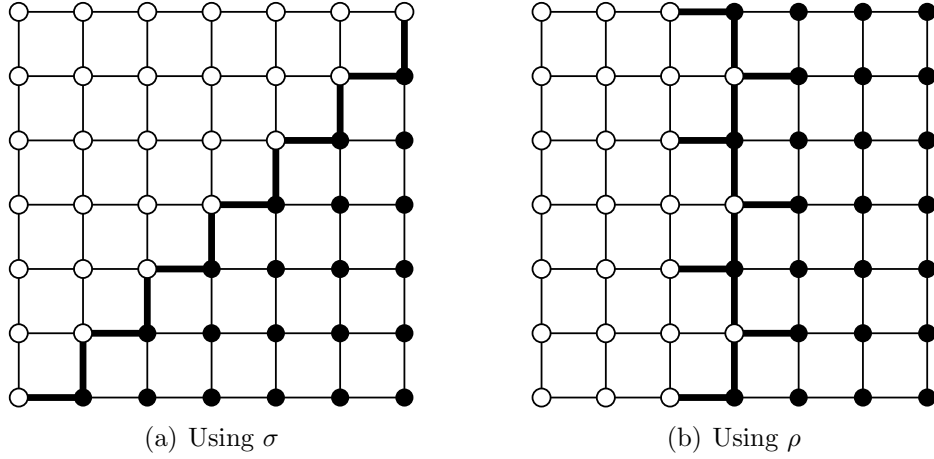
Figure 4.7: Two cuts (A, \bar{A}) described by the two discussed decompositions (T, \delta)_\sigma and (T, \delta)_\rho of a 7 \times 7 grid. The edges across the cut are drawn bold, vertices of A are white while vertices of \bar{A} are black.
